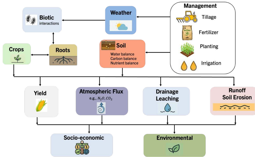
Figure 1 Process-based SALUS schematic (Basso et al., 2025b).
