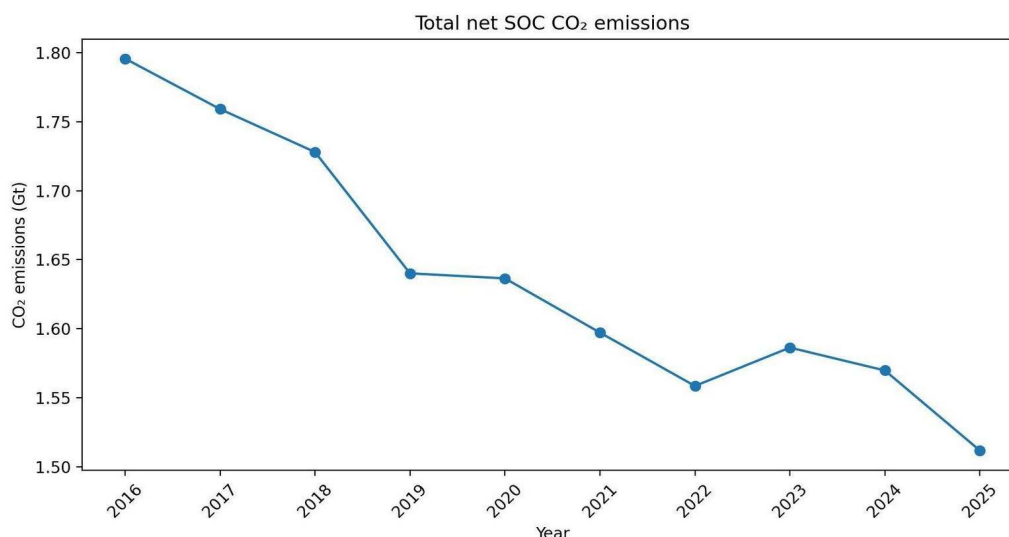
Figure 4 Global baseline net SOC emissions, 2016–2025 ( \text{Gt CO}_2 ).
