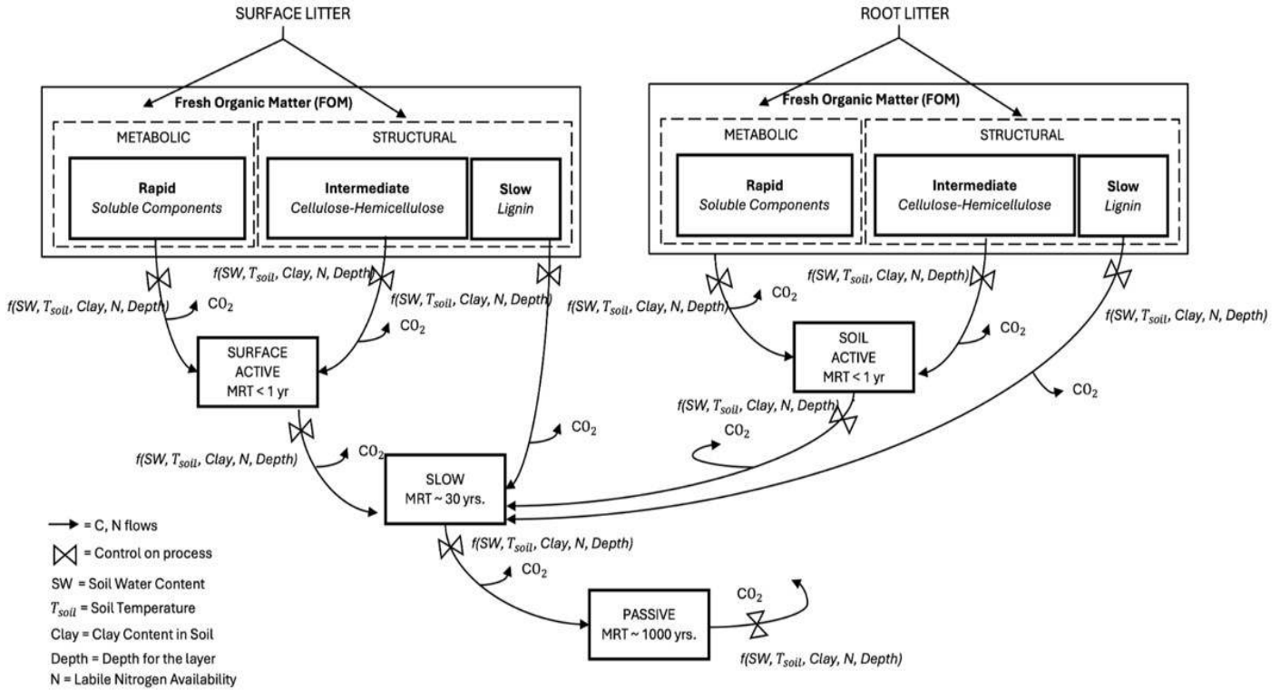
Figure 2 SALUS Soil Organic Carbon dynamics (Basso et al. 2015; Basso et al. 2025b).
